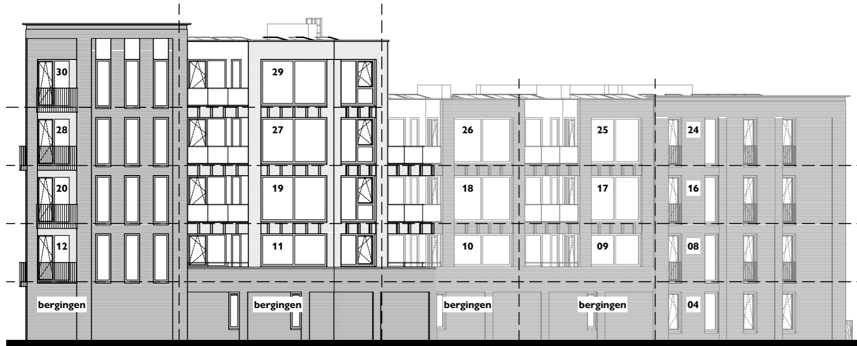
Westgevel links
